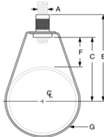
1 1/4" through 8" pipe
