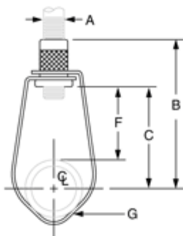
1/2" through 1" pipe
